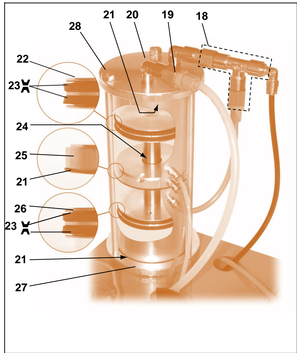
Overview cylinder
